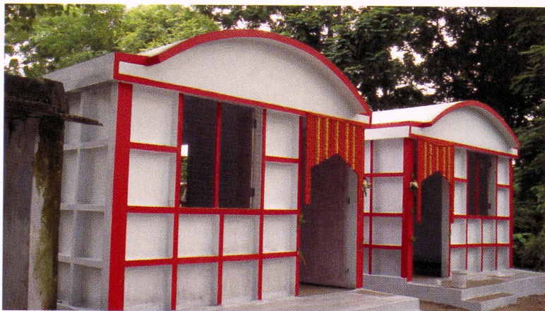
Completed one room kitchen house in ferrocement
