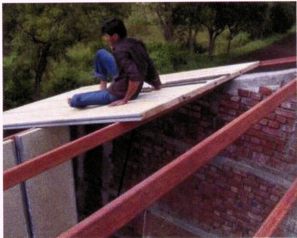
Wood wool board construction
