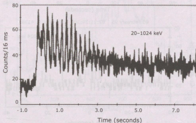
Figure 1. Light curve of a gamma-ray burst-like event, detected by SROSS-C GRB experiment on 29 June 1992. Oscillations with a period of 237 ms can be seen clearly.
