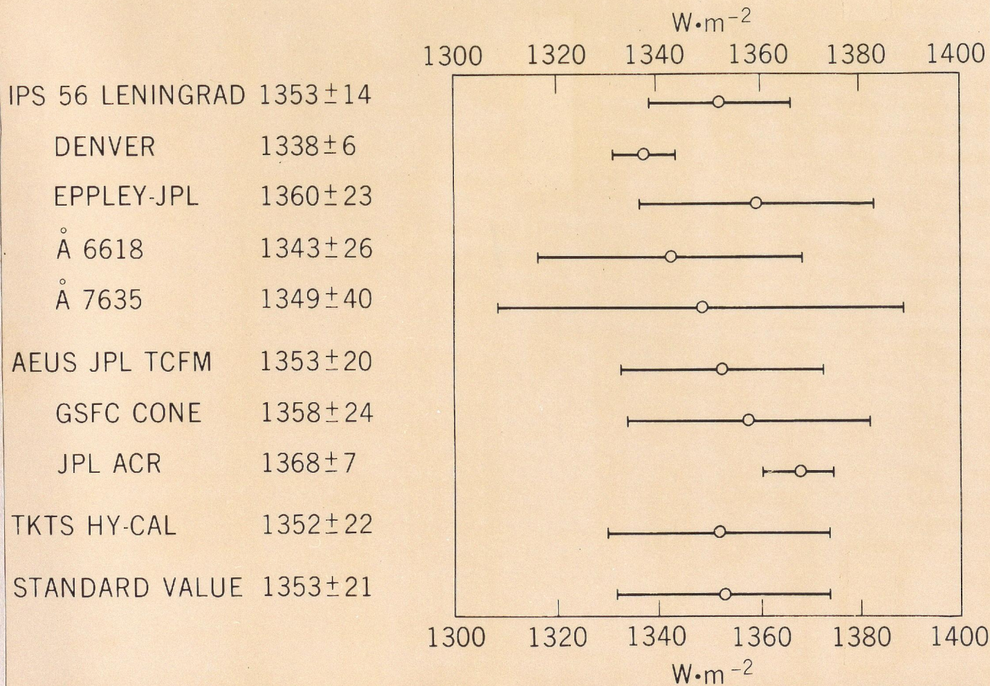
Figure 1. Values of solar constant derived from high altitude measurements
