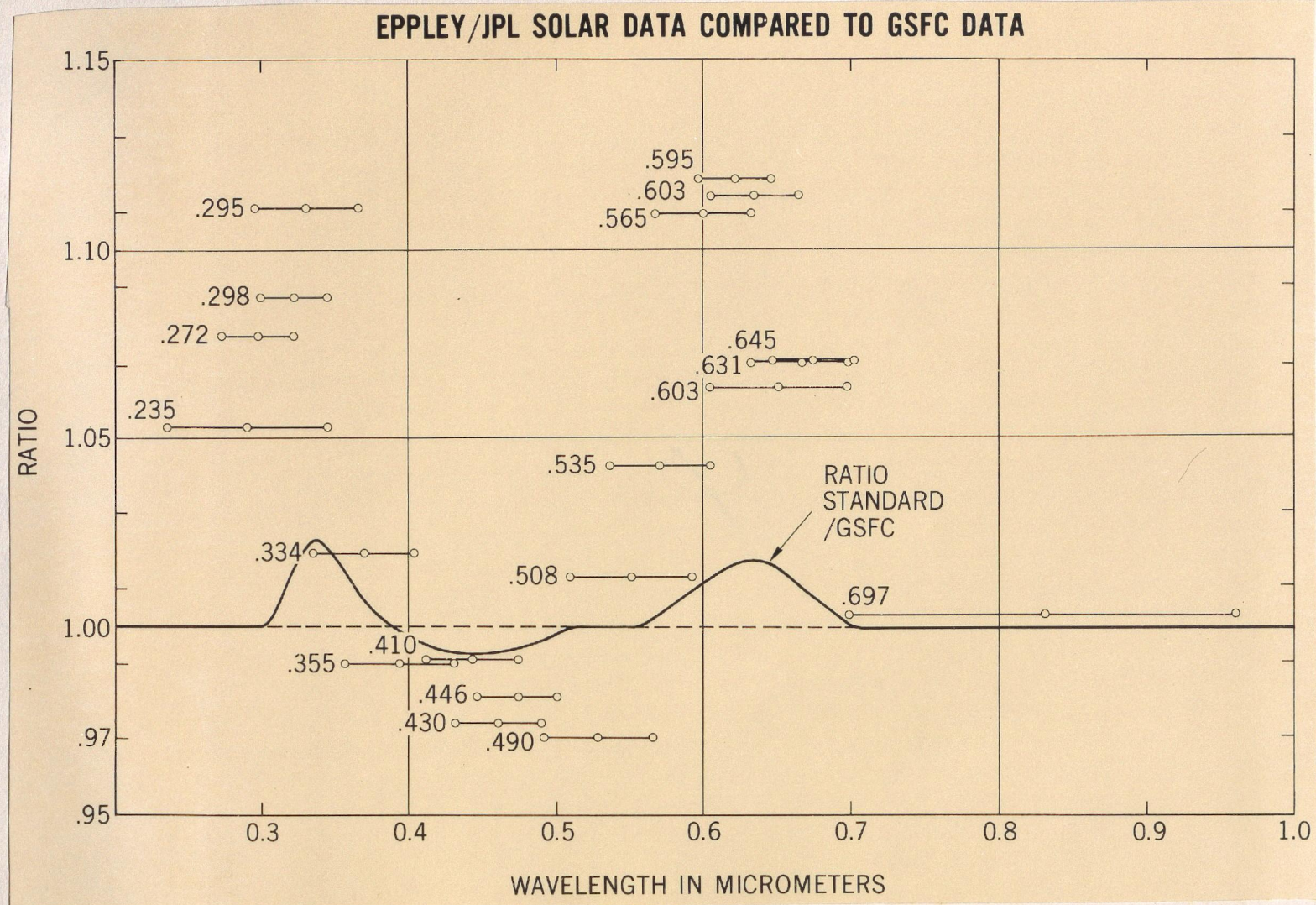
Figure 4. Comparison of Eppley JPL solar irradiance filter data with the GSFC CV990 monochromator spectral data
