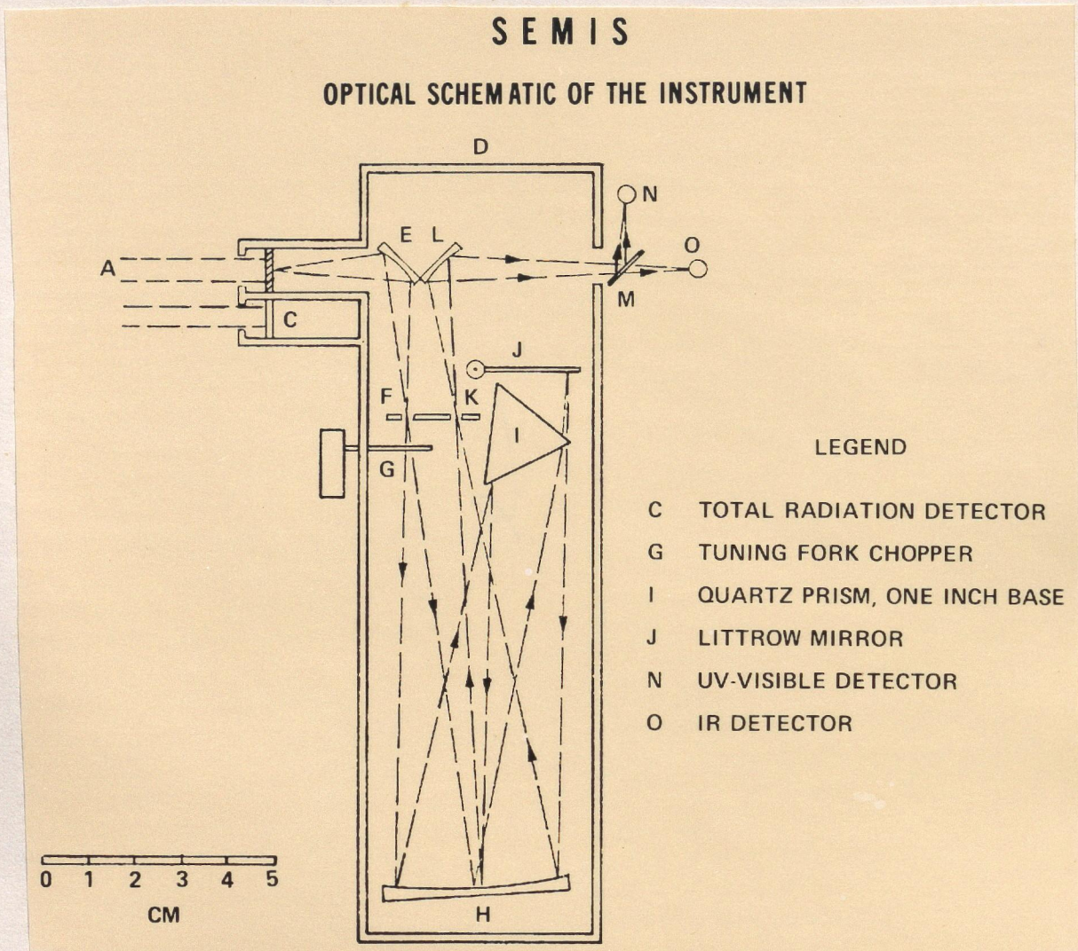
Figure 6. Optical schematic of SEMIS (Solar Energy Monitor in Space)
