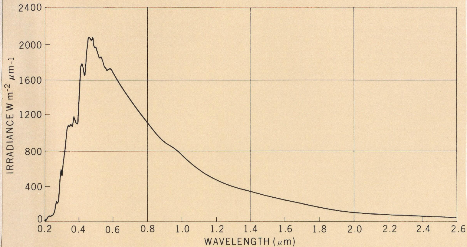
Figure 2. The NASA/ASTM standard curve of extraterrestrial solar spectral irradiance
