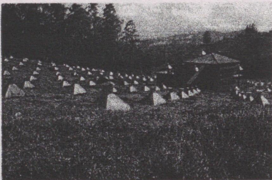
FIG. 4 Triple setup of Air Cerenkov Counter, multiplate Cloud Chamber and Total Absorption Spectrometer at Ooty, for the study of interactions of pions and protons in 10-40 GeV range.
