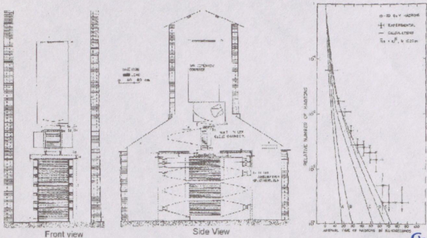
Figure 4. Triple arrangement of Air Cerenkov, Multiplate Cloud Chamber and Total Absorption Spectrometer at Ooty, for the study of interactions of pions and protons in 10-100 GeV range.
